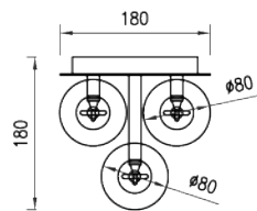
3 Plan View Scale 1:10
