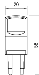
4 G9 Lamp Scale NTS
